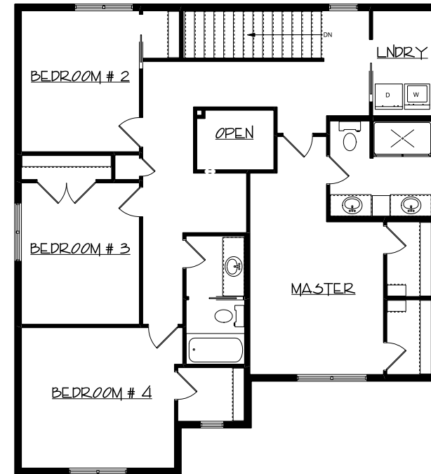
UPPER LEVEL 1,288 SQ FT
